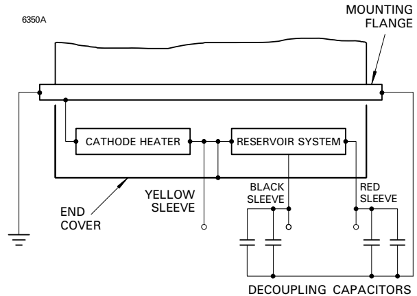
Fig. 2 CX1525AX, CX1525AWX base connections
