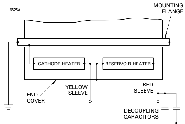
Fig. 1 CX1525A, CX1525AW base connections
