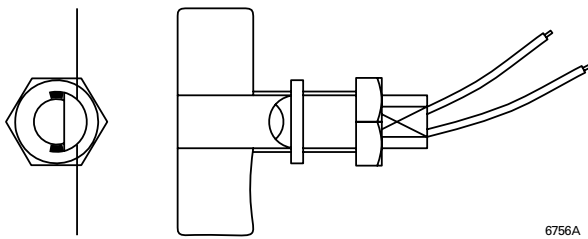
Fig. 3. Fan stop detection device
