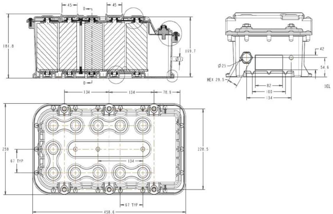
Figure 2: Dimensions
