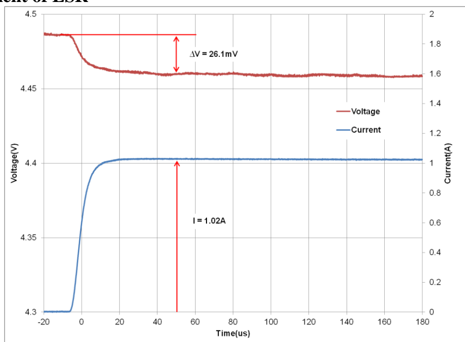
Fig 3: Measurement of ESR for a GS230
