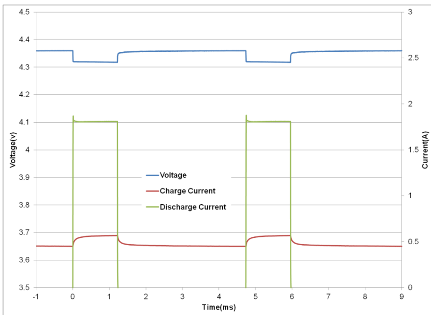
Fig 5: GS230 Pulse Response with GPRS Class 10 Pulse Train
