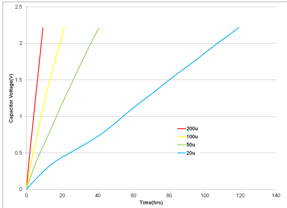
Fig 11: Charging an GS130 with low current
