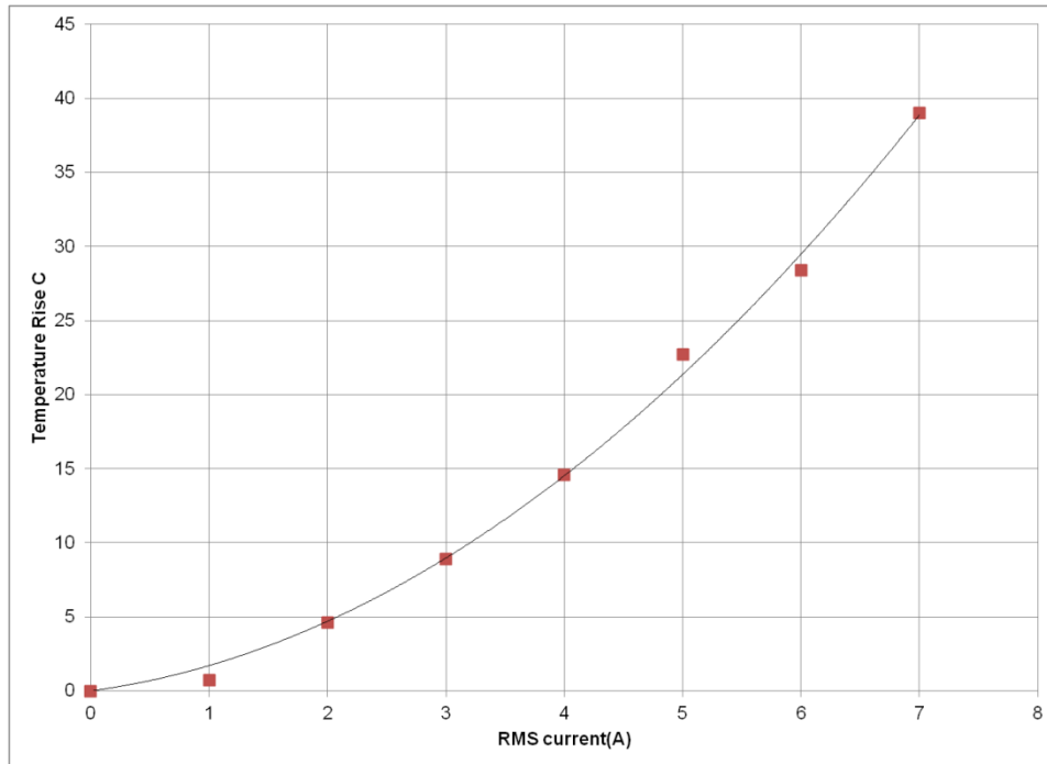
Fig 12: Temperature rise in GS230 with RMS current
