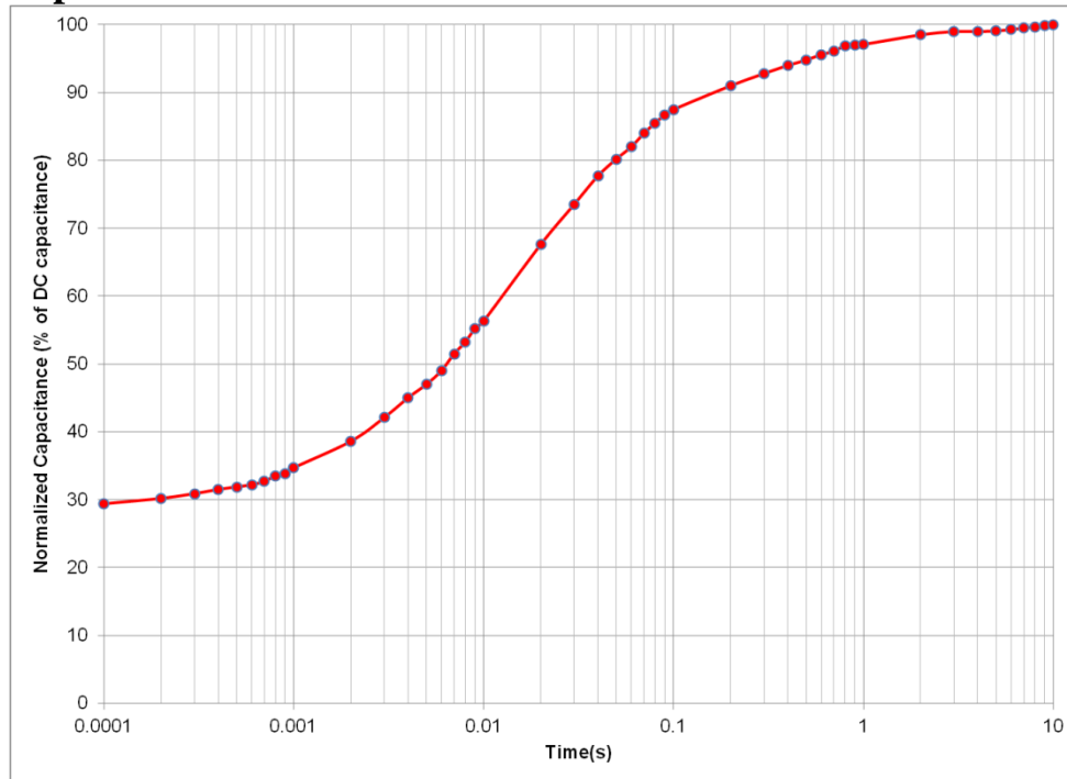
Figure 4: Effective Capacitance
