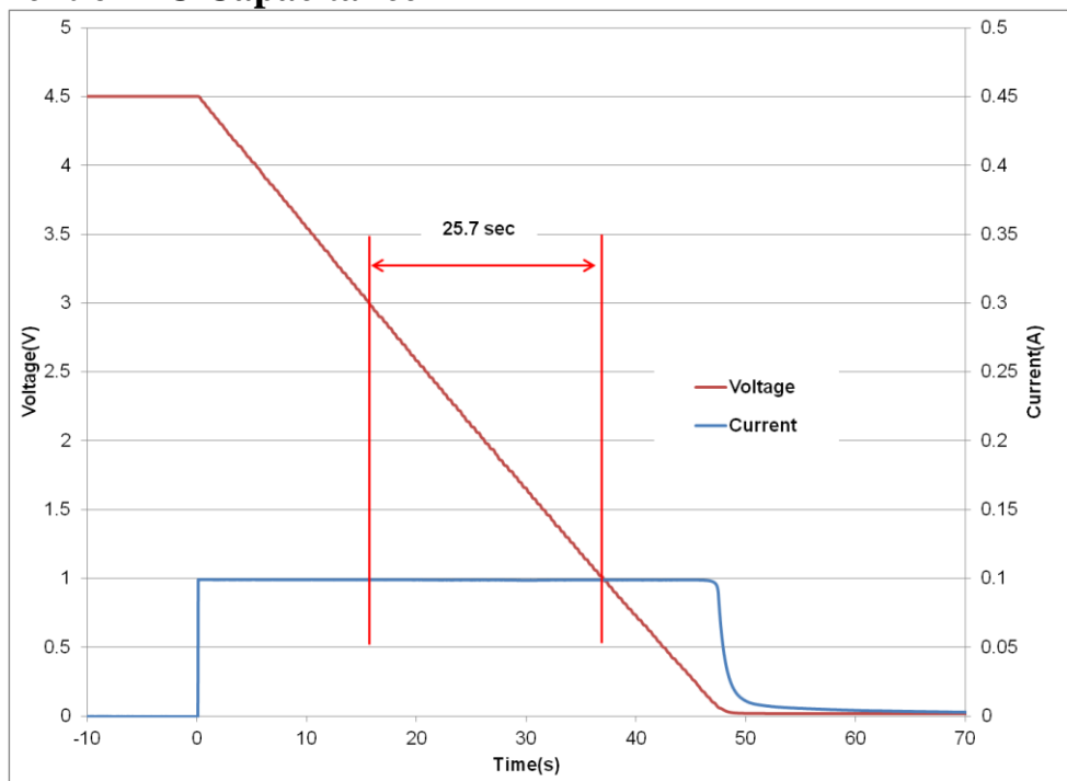
Fig 2: Measurement of DC Capacitance for a GS230
