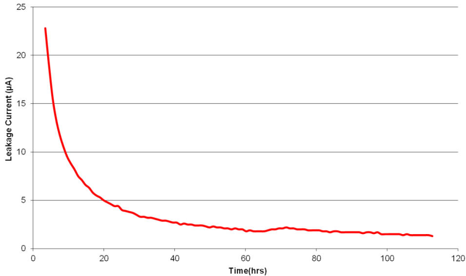
Fig 10: Leakage Current
