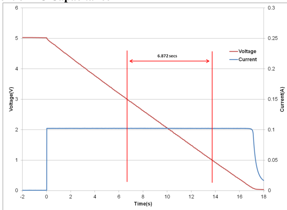
Fig 2: Measurement of DC Capacitance for an HW201
