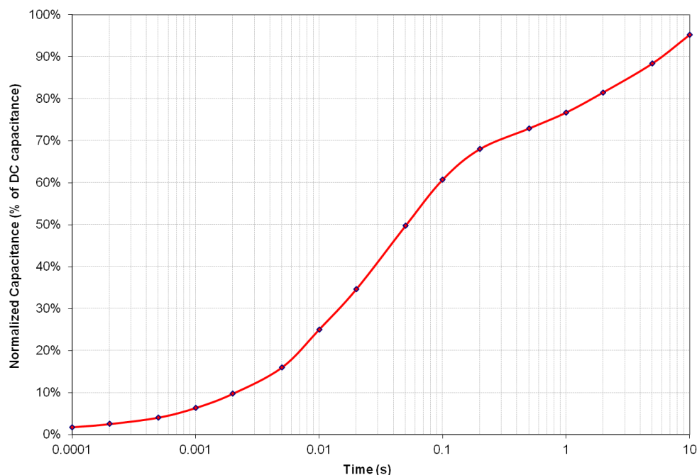
Figure 4: Effective Capacitance
