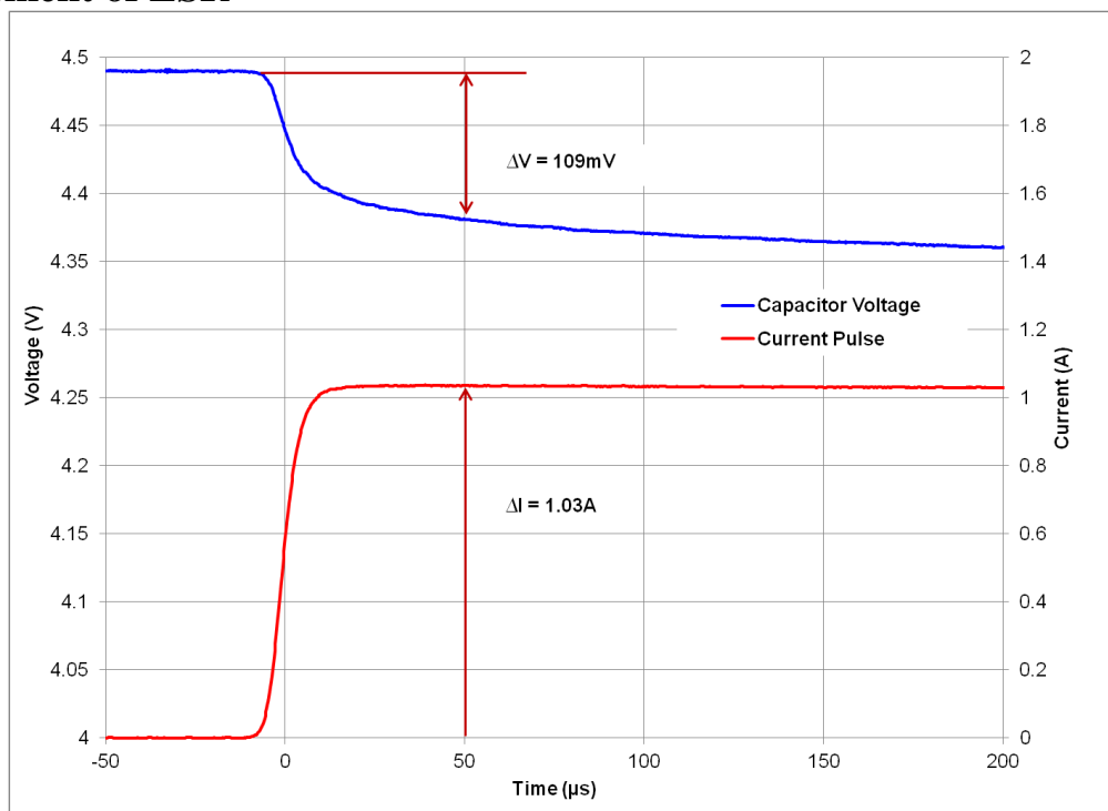
Fig 3: Measurement of ESR for an HW201
