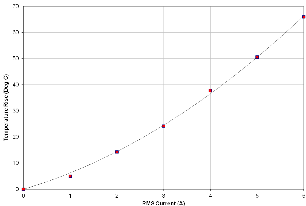
Fig 12: Temperature rise in HW201 with RMS current
