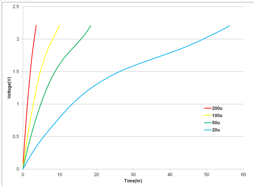
Fig 11: Charging an HW101 with low current
