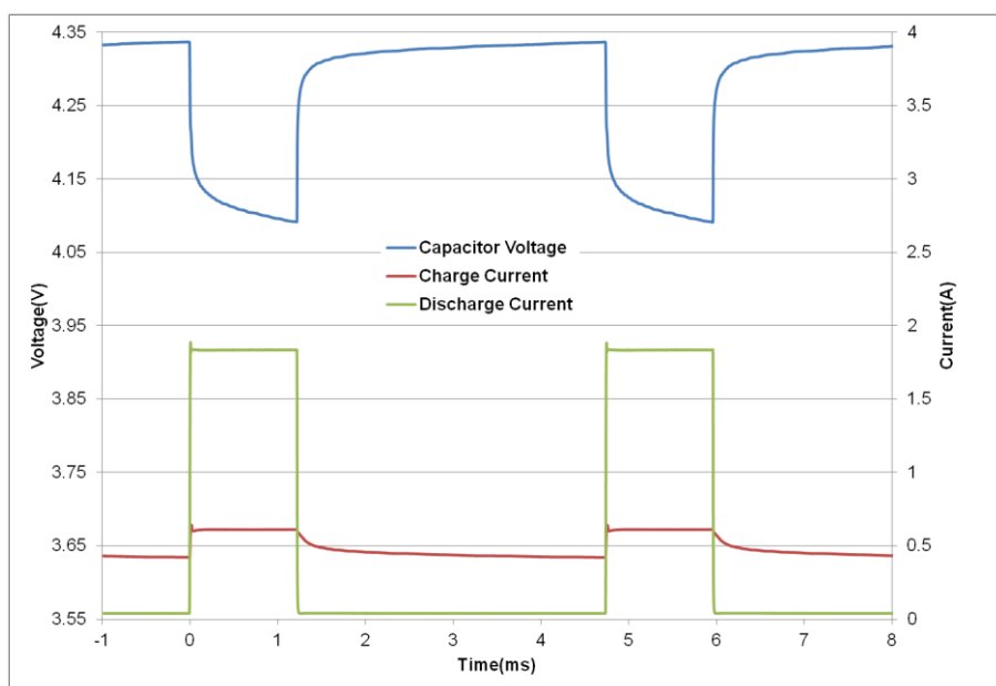
Fig 5: HW201 Pulse Response with GPRS Class 10 Pulse Train
