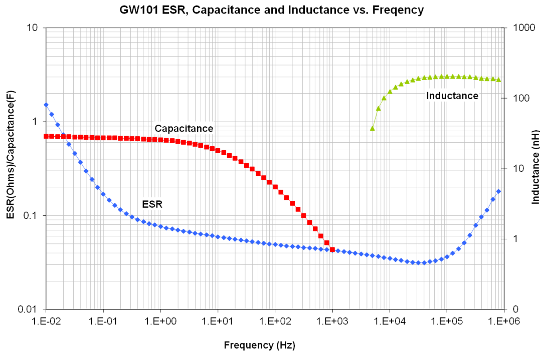
Fig 9: Frequency Response of ESR, Capacitance & Inductance
