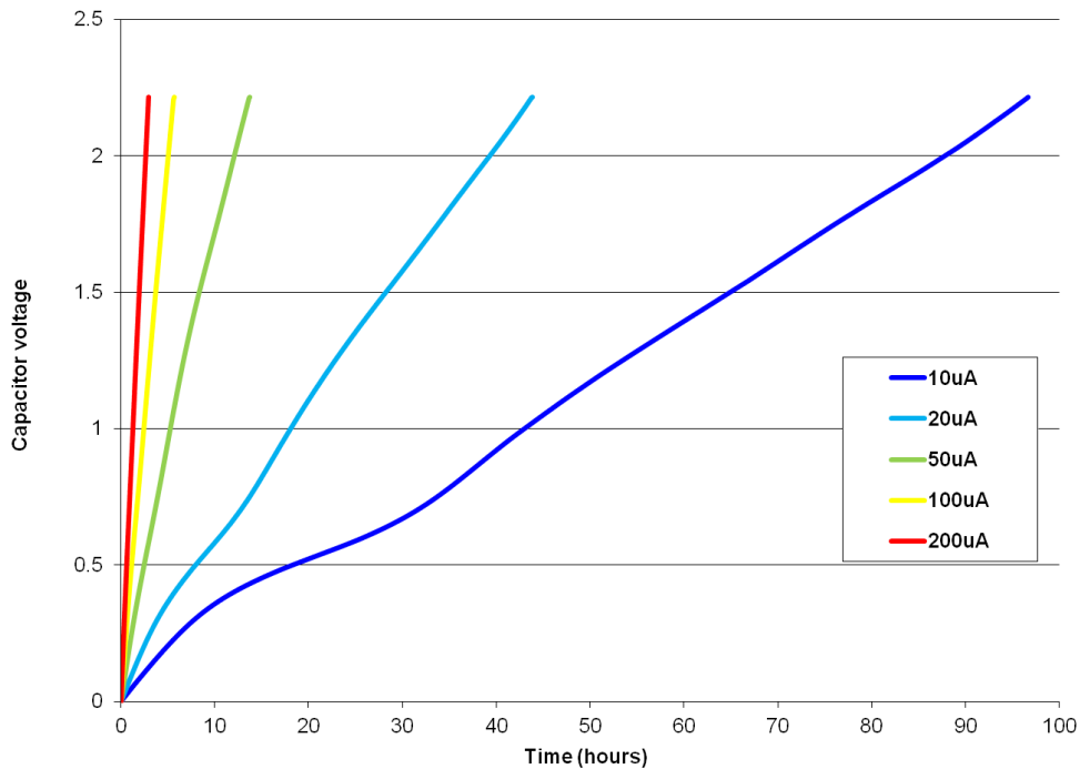
Fig 11: Charging an GW101 with low current
