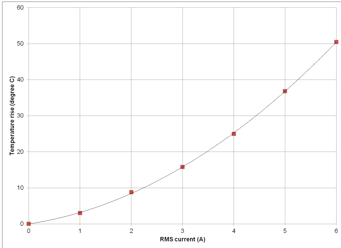
Fig 12: Temperature rise in GW201 with RMS current
