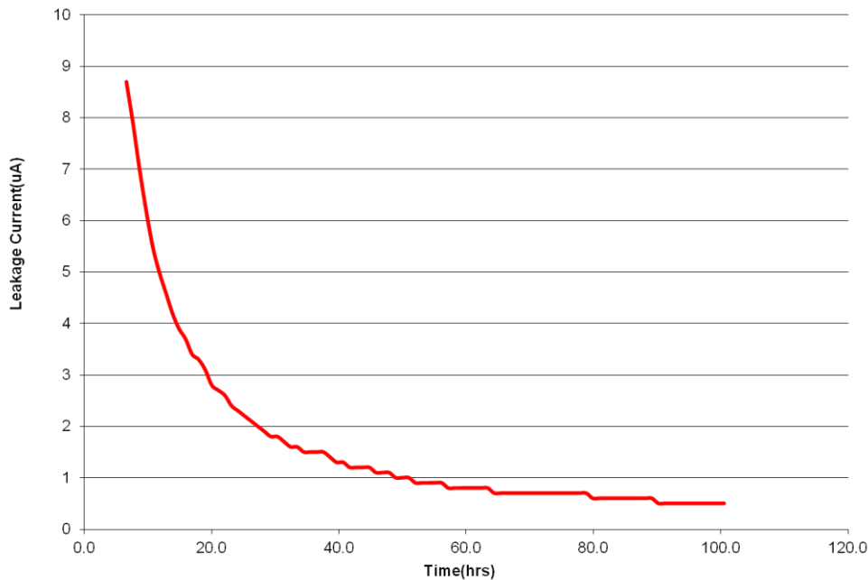
Fig 10: Leakage Current
