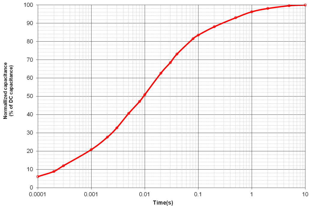
Figure 4: Effective Capacitance
