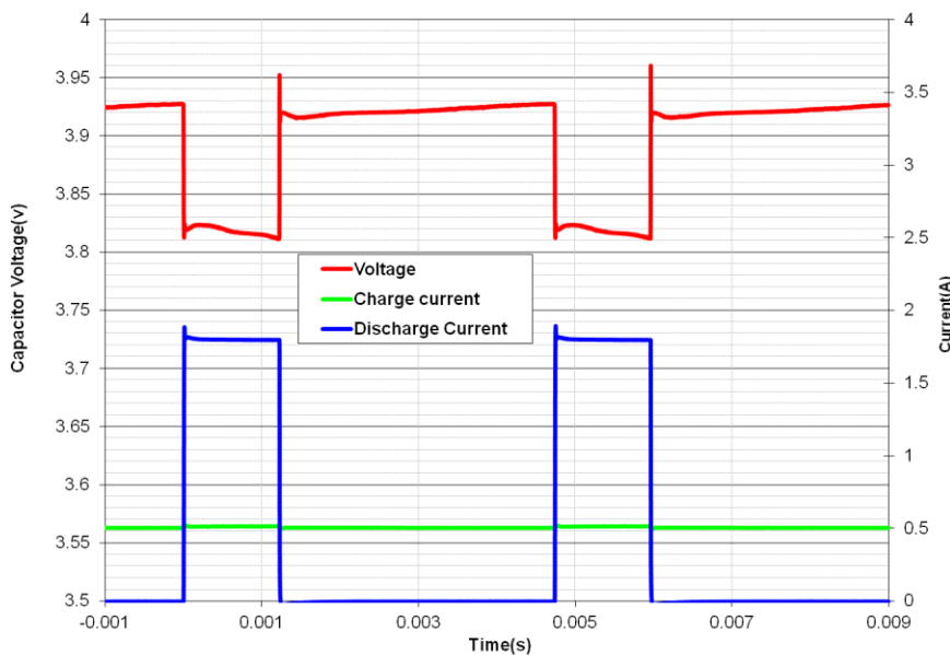
Fig 5: GS203 Pulse Response with GPRS Class 10 Pulse Train
