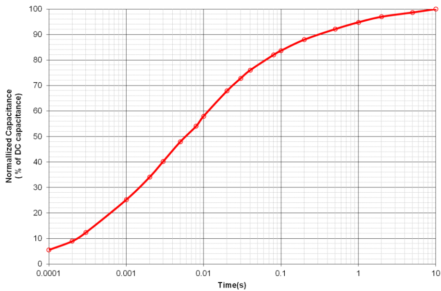
Figure 4: Effective Capacitance
