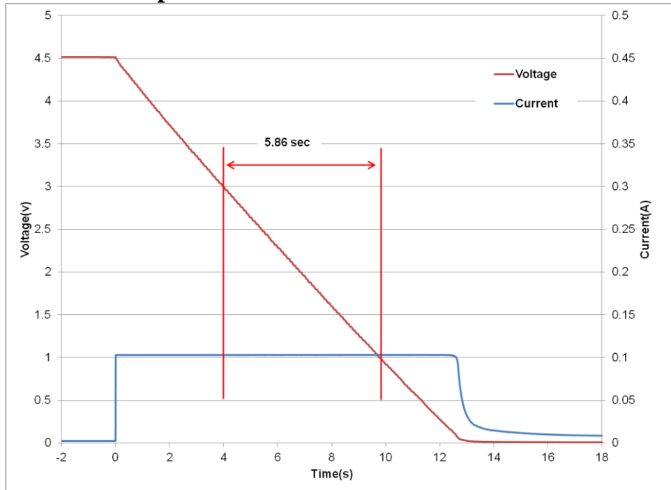
Fig 2: Measurement of DC Capacitance for a GS203
