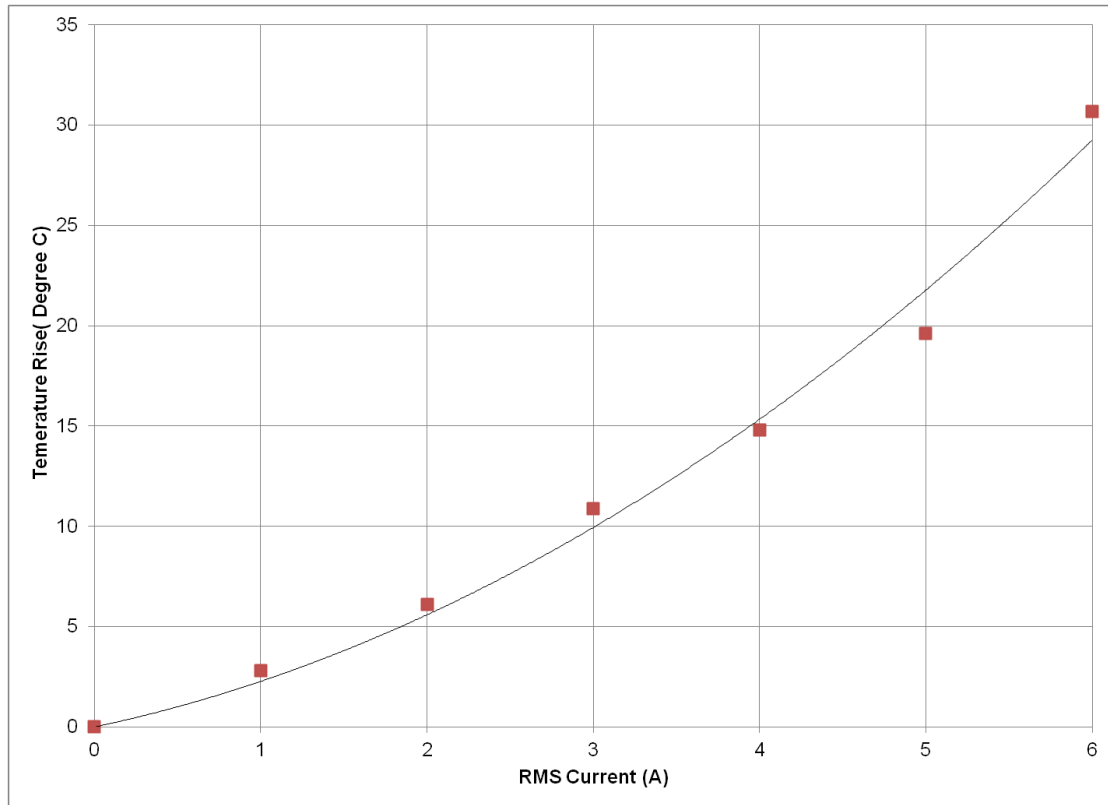
Fig 12: Temperature rise in GS203 with RMS current
