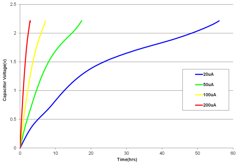
Fig 11: Charging a GS103 with low current
