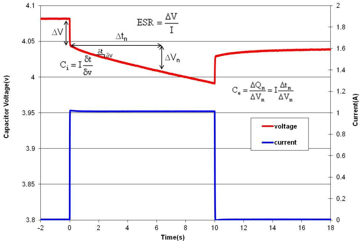
Figure 1: Effective capacitance, instantaneous capacitance and ESR for a GS203
