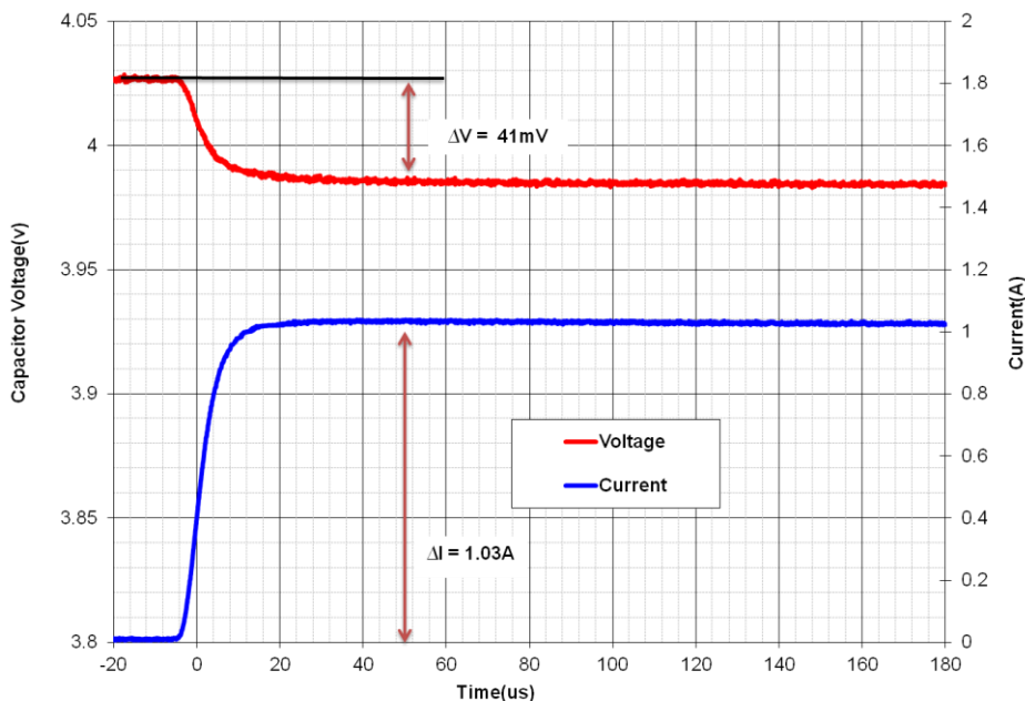
Fig 3: Measurement of ESR for a GS203
